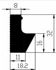
Order No. Mixture Nozzle VP7469 EPDM 50 DET
