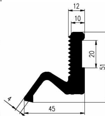
Order No. Mixture Nozzle VP4709 EPDM 70 ATV
