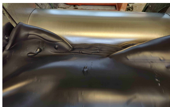
Calendering
