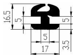
Order No. Mixture Nozzle VP6721 EPDM 70 CKZ
