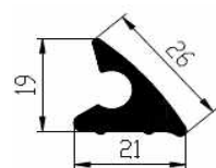
Order No. Mixture Nozzle VP7261 EPDM 70 CZB
