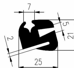
Order No. Mixture Nozzle VP5223 EPDM 60 BFP
