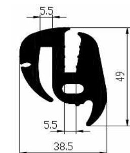
Order No. Mixture Nozzle VP7224 EPDM 45 CYA
