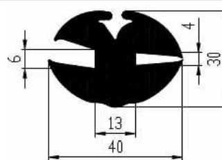
Order No. Mixture Nozzle VP6468 EPDM 60 CFB
