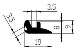
Order No. Mixture Nozzle VP6280 EPDM 50 BZZ-II
