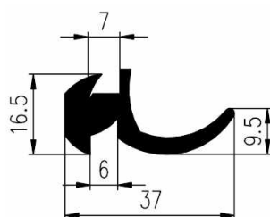
Order No. Mixture Nozzle VP3672 EPDM 70 ZS
