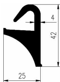
Order No. Mixture Nozzle VP4619 EPDM 65 ASN
