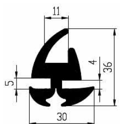
Order No. Mixture Nozzle VP5955 EPDM 70 BTN
