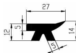
Order No. Mixture Nozzle VP4477 NBR 60 APC
