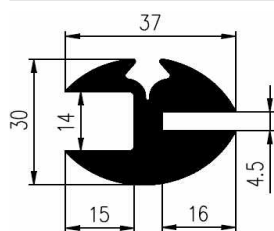
Order No. Mixture Nozzle VP4249 EPDM 70 AKL
