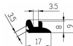
Order No. Mixture Nozzle VP6236 EPDM 50 BZZ-I
