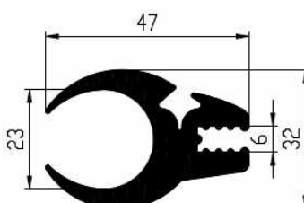
Order No. Mixture Nozzle VP5714 EPDM 65 BOL
