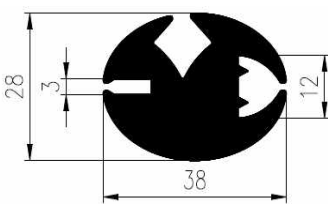
Order No. Mixture Nozzle VP3372 EPDM 70 VQ
