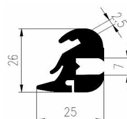
Order No. Mixture Nozzle VP5403 EPDM 70 BIX
