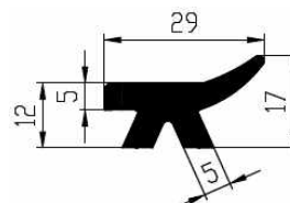
Order No. Mixture Nozzle VP5856 NBR 60 BRN
