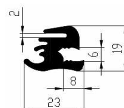
Order No. Mixture Nozzle VP6761 EPDM 60 CLW
