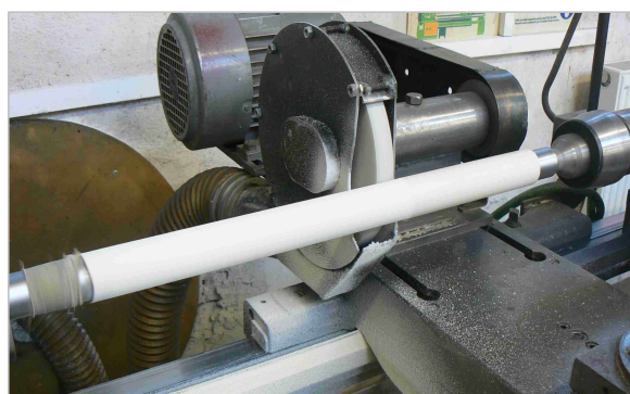
Hose grinding
