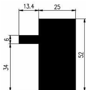
Order No. Mixture Nozzle VP2095 NBR 70 IA
