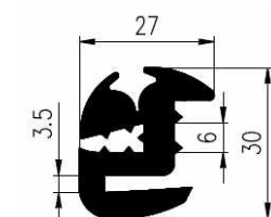
Order No. Mixture Nozzle VP5259 EPDM 70 BBH
