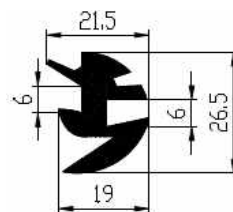
Order No. Mixture Nozzle VP6514 EPDM 70 CGG
