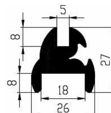
Order No. Mixture Nozzle VP5708 EPDM 70 BOI
