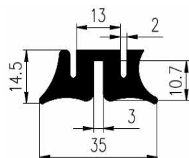
Order No. Mixture Nozzle VP4335 EPDM 70 AMK
